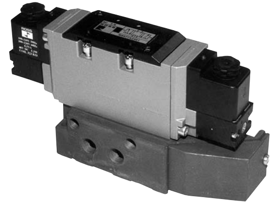
Base-Mount
